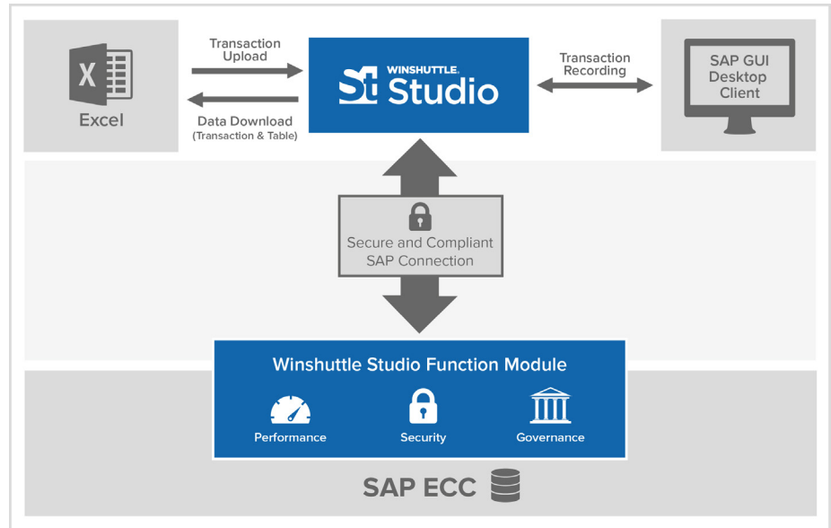
Winshuttle Studio architecture
